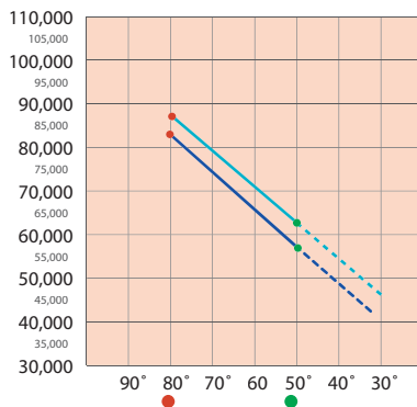
H100R HEATING BTU RATING PER HOUR
