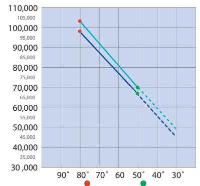
H120R HEATING BTU RATING PER HOUR
